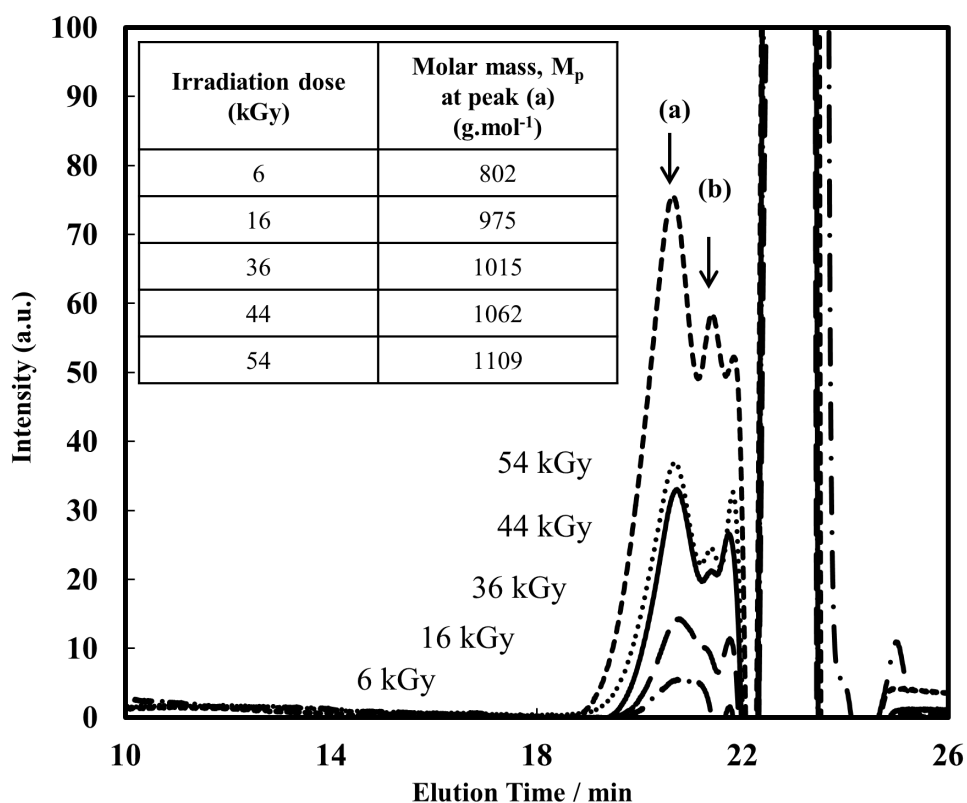
Figure 2. SEC chromatograms of PEDOT polymers synthesized in DCM under N_2 by \gamma -radiolysis at increasing doses. The initial concentration of EDOT was 10 mM.
