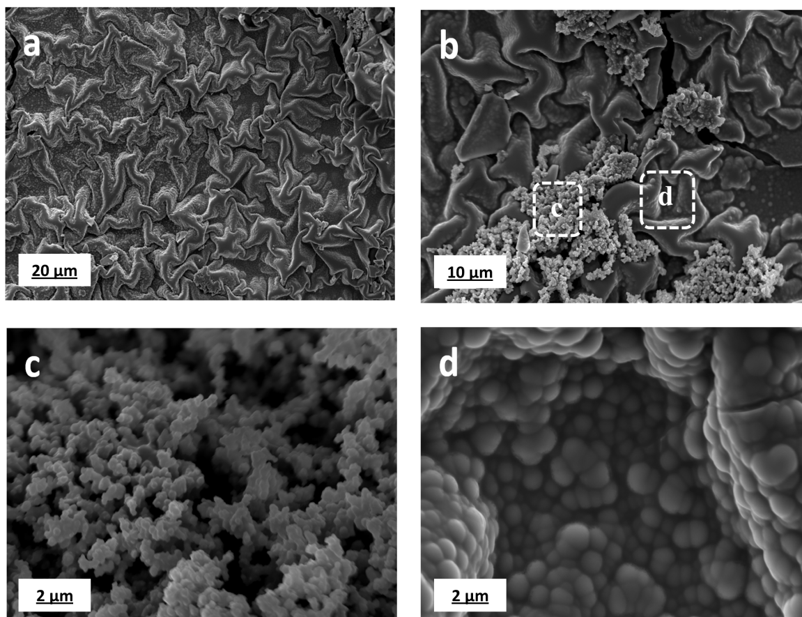
Figure 6. SEM images of dried PEDOT polymers powder after deposition onto carbon tape adhered to aluminum mounts and gold coating. The powder was obtained after solvent evaporation. PEDOT polymers were synthesized by gamma-radiolysis at 36 kGy of a DCM solution containing 10 mM in EDOT under N_2 atmosphere.
