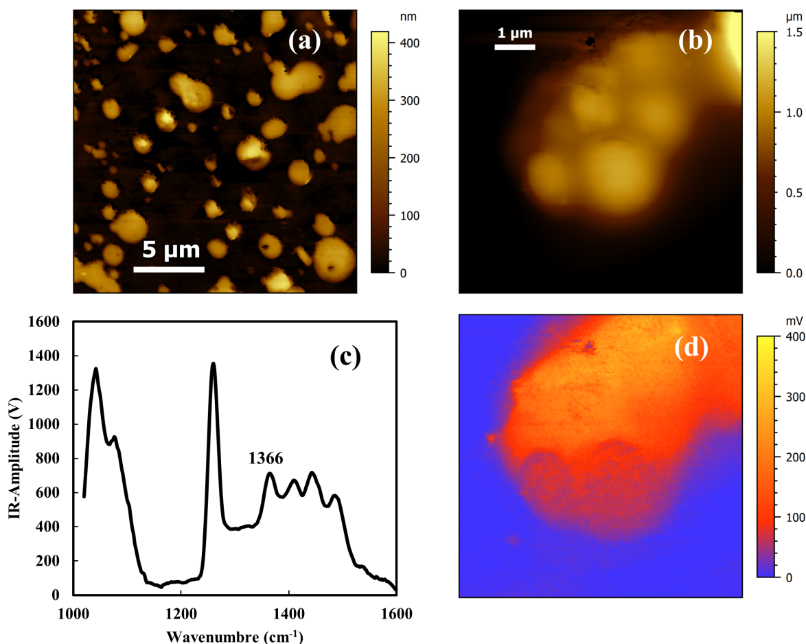
Figure 7. AFM-IR images of PEDOT polymers after deposition onto the upper surface of ZnSe prism. PEDOT polymers were synthesized by gamma-radiolysis at 36 kGy of a DCM solution containing 10 mM in EDOT under N_2 atmosphere. (a) and (b) AFM topographic images of PEDOT polymers in contact mode. (c) AFM-IR spectrum of PEDOT. (d) AFM-IR chemical mapping of PEDOT with the IR source tuned to the C-C band at 1366\text{ cm}^{-1} .
