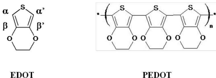
Scheme 1. Chemical structures of 3,4-ethylenedioxythiophene (EDOT) and poly(3,4-ethylenedioxythiophene) (PEDOT). EDOT structure displays the free \alpha , \alpha' positions where polymerization could occur.
