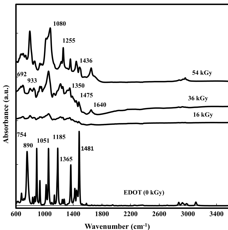
Figure 3. ATR-FTIR spectra of pure EDOT monomers and of PEDOT polymers radiolytically synthesized in DCM solvent in presence of 10 mM in EDOT at irradiation doses of 16, 36 and 54 kGy under \text{N}_2 atmosphere.
