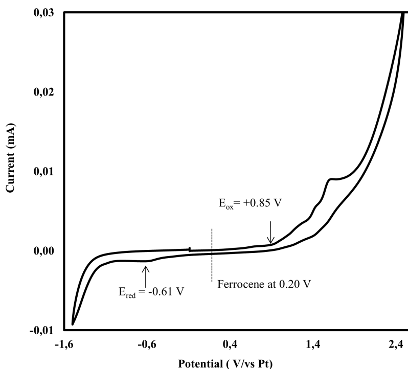
Figure 9. Cyclic voltammogram of PEDOT polymers recorded in acetonitrile containing 0.1 M of TBAPF_6 at a scan rate of 20 mV/s. PEDOT polymers were radiosynthesized at 36 kGy in a DCM solution containing 10 mM in EDOT under N_2 atmosphere. Ferrocenium/ferrocene ( Fc^+/Fc ) redox potential was measured in order to calibrate the pseudo reference electrode (0.2 V vs. Pt in the present study). The HOMO/LUMO energetic levels of PEDOT are determined as follows: E_{HOMO} (eV) from ionization potential = -4.8-e ( E_{ox}-0.2 ) and E_{LUMO} (eV) from electronic affinity = -4.8-e ( E_{red}-0.2 ) where e is the elementary charge.
