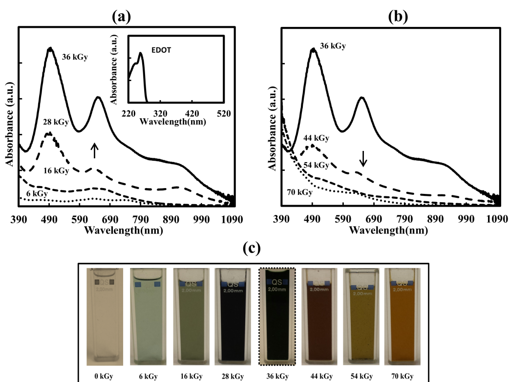
Figure 1. UV-Vis absorption spectra of DCM solutions containing 10 mM in EDOT and irradiated under N_2 atmosphere at increasing doses from: (a) 0 to 36 kGy and (b) from 36 to 70 kGy. The reference was DCM. (c) Photographs of DCM solutions before and after irradiation at increasing doses.
