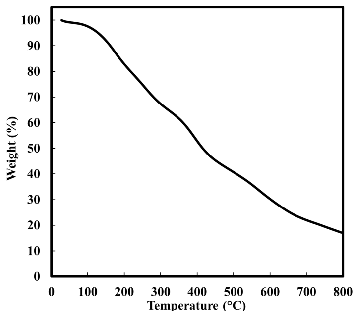
Figure 8. Thermogravimetric analysis (TGA) graph of dried PEDOT polymers powder. The polymers were synthesized by gamma-radiolysis at 36 kGy of a DCM solution containing 10 mM in EDOT under N_2 atmosphere.
