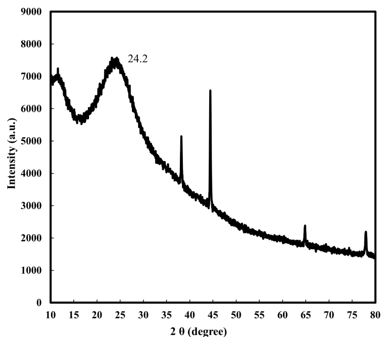
Figure 5. XRD pattern of dried PEDOT polymers powder obtained after DCM evaporation. The polymers were synthesized by gamma-radiolysis at 36 kGy of a DCM solution containing 10 mM in EDOT under N_2 atmosphere. The substrate used for XRD analysis was aluminium.
