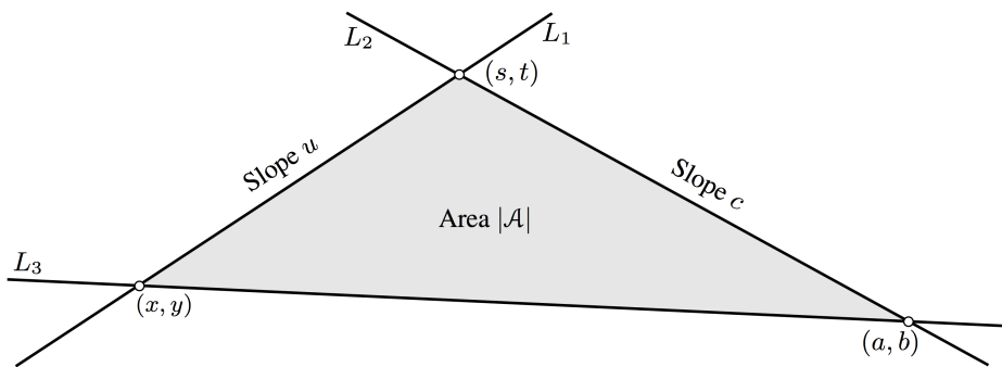
FIGURE 1. Geometric construction of the joint invariant \mathcal{A} .
