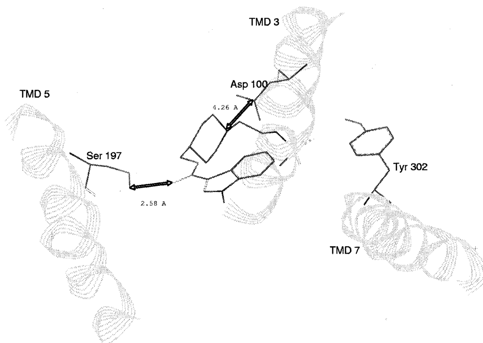
Figure 9 GR113808-h5-HT 4 receptor complex model. It is characterized by distances: (i) d = 2.58 Å between the hydroxylic hydrogen of S197(5.43) and the GR113808 carbonyl oxygen, (ii) d = 4.26 Å between the carboxylic carbon of D100(3.32) and the GR113808 basic nitrogen.
