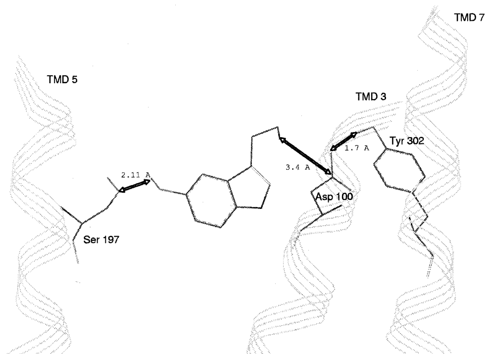
Figure 8 Serotonin-h5-HT 4 receptor complex model. Obtained by docking experiment, this model is characterized by distances: (i) d = 2.11 Å between the hydroxylic oxygen of S197(5.43) and the serotonin hydroxylic hydrogen, (ii) d = 3.4 Å between the carboxylic carbon of D100(3.32) and the serotonin basic nitrogen, and (iii) d = 1.7 Å between the carboxylate oxygen in D100(3.32) and the phenolic hydrogen of Y302(4.43).
