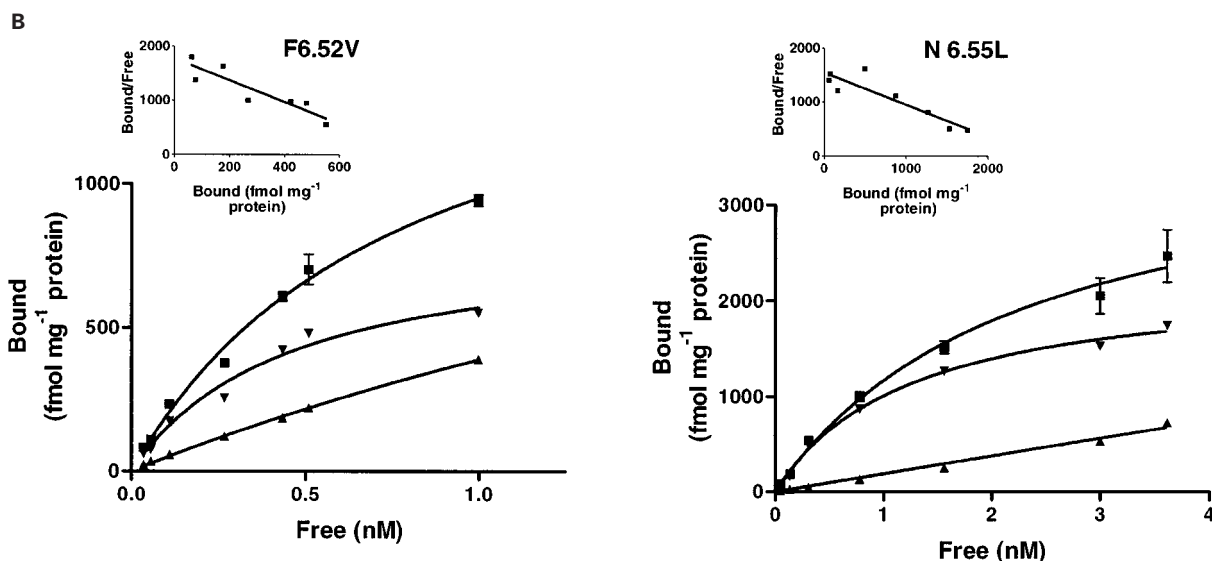
Figure 4 Saturation analysis of [ ^3\text{H} ]-GR113808 binding to COS-7 cells transfected with wild-type or mutant human h5-HT 4(a) receptors. Non-specific binding was determined with 10 \mu\text{M} ML10375. Experiments were performed in triplicate using a range of nine concentrations of radioligand.
