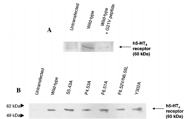
Figure 6 Protein immunoblotting of the mutant and wild type h5-HT 4(a) receptors expressed in COS-7 cells. Plasma membrane protein extracts were separated on a polyacrylamide gel and analysed by immunoblotting with antiserum against the second extracellular loop of h5-HT 4(a) receptor (see methods). (A) COS-7 cells were transfected with the wild-type h5-HT 4(a) receptor (lane 2 and lane 3) or the corresponding control (lane 1). The immunoreactivity of wild-type receptor was blocked by incubation with a peptide (G21V) corresponding to the second extracellular loop of the receptor (lane 3). (B) In COS-7 cells transfected with the wild-type h5-HT 4 receptor (lane 2) and different mutants (lane 3–7), a specific band migrating to the level of 60 kDa was detected whereas in non transfected control cells (lane 1) no labelling was detected at this position.
