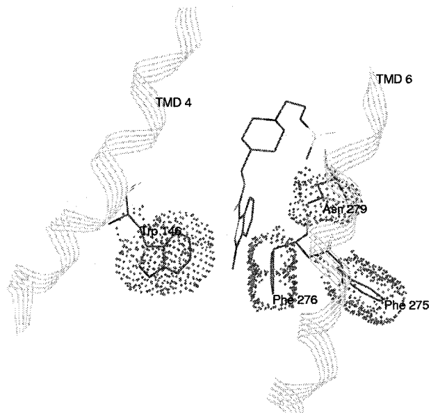
Figure 10 Representation of hydrophobic interactions between the indol ring of GR113808 and a pocket constituted by W146(4.46), F275(6.51), F276(6.52) and N279(6.55).
