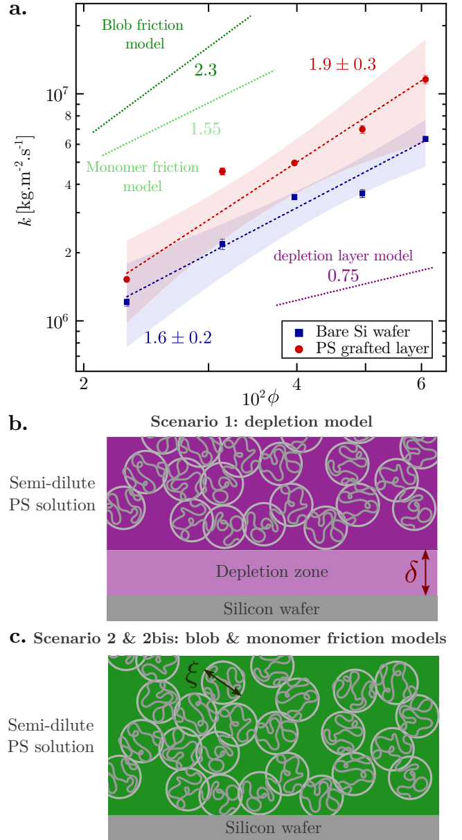
Figure 4: (a) Navier's coefficient k = b_{\infty}/\eta as a function of PS volume fraction \phi for solutions of PS in DEP flowing on a bare Si wafer and a grafted layer of PS brushes. The red and blue dotted lines represent fits b_{\infty} \propto \phi^{\beta} . The green and purple dotted lines correspond to the expected scaling laws according respectively to the blob friction model, the monomer friction model or the depletion layer model. (b) Illustration of the depletion model (scenario 1). \delta is the thickness of the depletion layer. (c) Illustration of the blob friction model (scenario 2) and the monomer friction model (scenario 2bis). \xi is the blob size.
