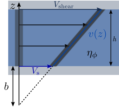
Figure 1: Definition of the slip length b measured by velocimetry using photobleaching. A drop of homogeneous polymer solution of viscosity \eta_\phi and thickness h , sheared at a velocity V_{\text{shear}} , slips on the bottom surface with a slip velocity V_s . The length at which the extrapolation of the velocity profile v(z) reaches zero is called the slip length b .
