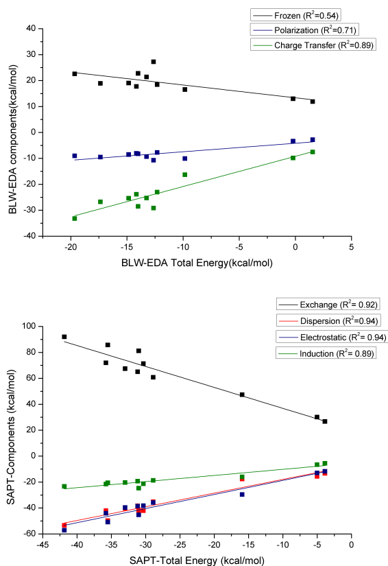
Fig. 11 The correlation of the respective energy decomposition terms with respect to the total energy for the various complexes: (top) BLW-EDA, and (bottom) SAPT.
