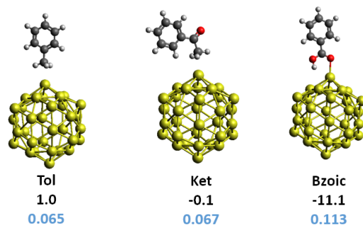
Fig. 5 Interaction of substituted aromatic compounds with Au 32 adopting perpendicular configuration of the aromatic ring, along with the interaction energy (in kcal/mol, black color) and the charge transfer with ADCH scheme (in e - , blue color).
