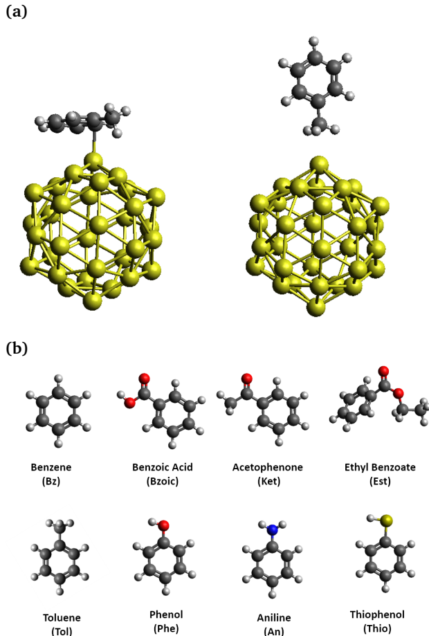
Fig. 1 (a) Schematic representation of aromatic compounds adsorbed on Au 32 adopting flat configuration "F" (left) or perpendicular configuration "P" (right). (b) Aromatic molecules and their abbreviations.
