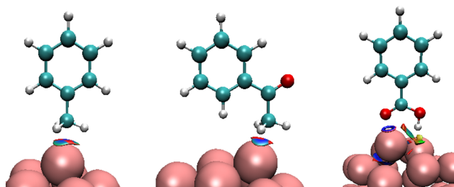
Fig. 8 NCI analysis of the aromatic molecules adsorbed on \text{Au}_{32} in a perpendicular configuration, see figure 7 for the color code: toluene, acetophenone, and benzoic acid
