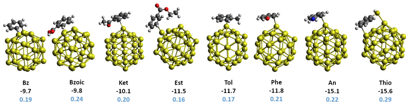
Fig. 3 Interaction of substituted aromatic compounds with Au 32 adopting a flat configuration of the aromatic ring, along with the interaction energy (in kcal/mol, black color) and the charge transfer with ADCH scheme (in e - , blue color).
