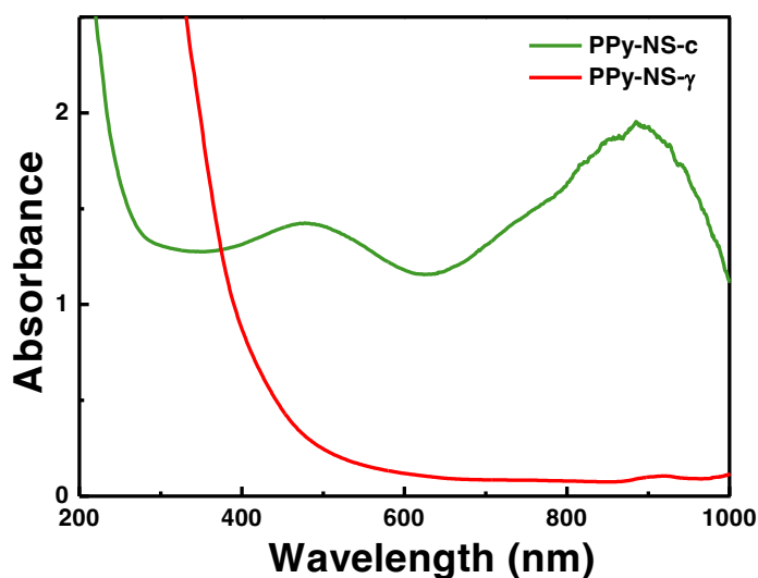
Fig. 5: UV-Vis spectra of the PPy nanostructures (PPy-NS-c and PPy-NS- \gamma ) and PPy-bulk in powder and in suspension.
