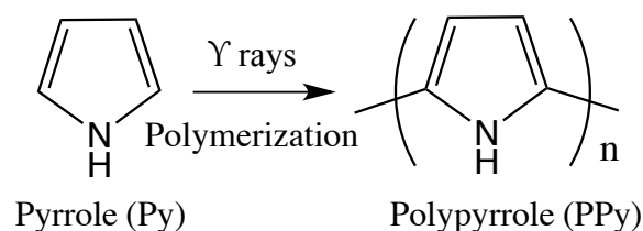
Scheme 1. PPy Polymerization by radiolysis.
