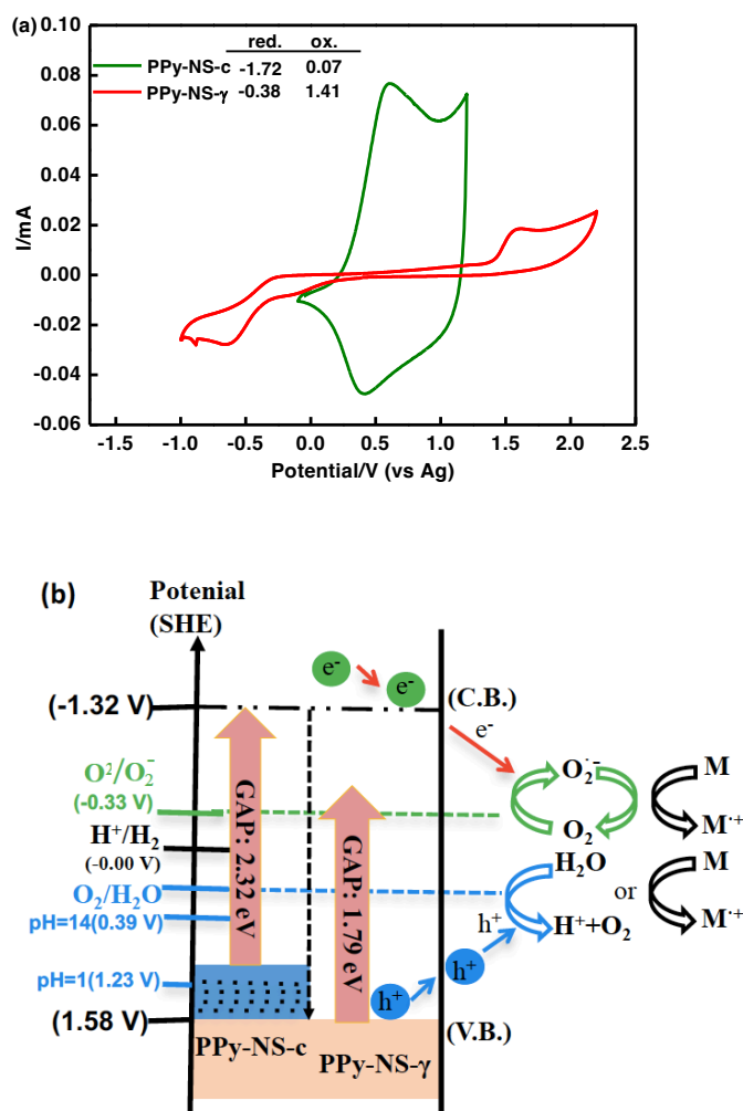
Fig. 8. (a) Cyclic Voltammetry of PPy recorded at 20 mV/s in acetonitrile and 0.1 M Tetrabutylammonium Perchlorate. Ferrocenium/ ferrocene (Fc/Fc + ) redox potential has been measured at the end of each experiment in order to calibrate the pseudo reference electrode (0.241 V vs. Ag in the present study). The energetic levels of PPy are obtained by the following equation: E_{\text{HOMO}} (\text{eV}) = - (4.8 + E_{\text{ox\_onset}} - 0.241) and E_{\text{LUMO}} (\text{eV}) = - (4.8 + E_{\text{red\_onset}} - 0.241) . (b) Possible photocatalytic mechanism with charge separation in PPy nanostructures with electron reducing oxygen and the hole oxidizing water.
