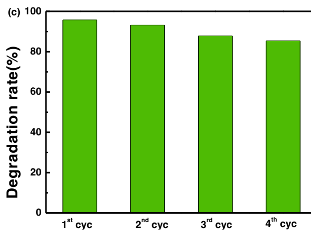
Fig. 6: Degradation rates of phenol in the presence of as-prepared samples of PPy under UV-Vis (a) and visible light irradiation (b) ; (c) Photocatalytic activity of PPy-NS-c with cycling.
