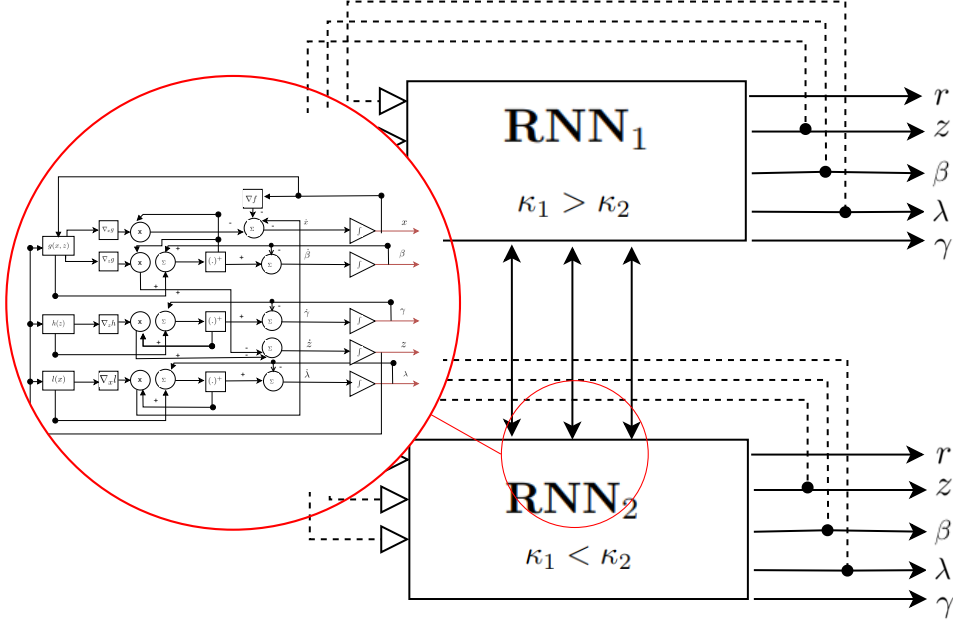
Figure 1: A block diagram depicting a duplex neurodynamic system with a two-timescale configuration
