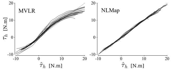
Fig. 7: Effect of mapping nonlinearization on Elbow torques. Comparison between MVLR and NLMap of reference ( \tau_h ) to estimated ( \hat{\tau}_h ) torques correlations. Each line corresponds to one participant and represents the smoothed data from the ten 30s trials.
