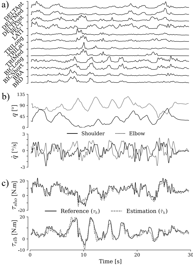
Fig. 5: Multi-joint torque estimation with the NLMap model for a representative participant. a) Processed EMG signals. b) Angular position and velocity of the Shoulder and Elbow. c) Shoulder ( \tau_{sho} ) and Elbow ( \tau_{elb} ) reference and estimated torques.
