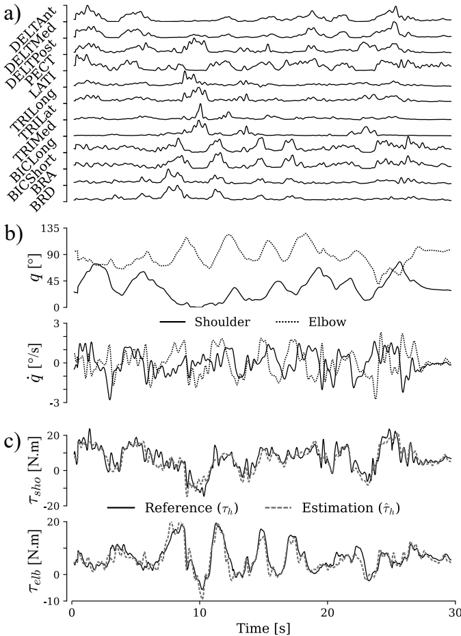
Fig. 7: Multi-joint torque estimation with the NLMap model for a representative participant. a) Processed EMG signals. b) Angular position and velocity of the Shoulder (solid) and Elbow (dotted). c) Shoulder ( \tau_{sho} ) and Elbow ( \tau_{elb} ) reference and estimated torques. Reference and estimated torques are respectively represented using a solid and a dashed line.
