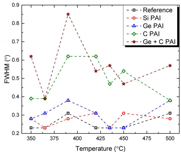
FIG. 9. Evolution of the FWHM values collected for the Ni mono-stanogermanide peak around 53.5 ° from various in situ XRD measurements for Ni/GeSn systems without and with various PAI treatments.
