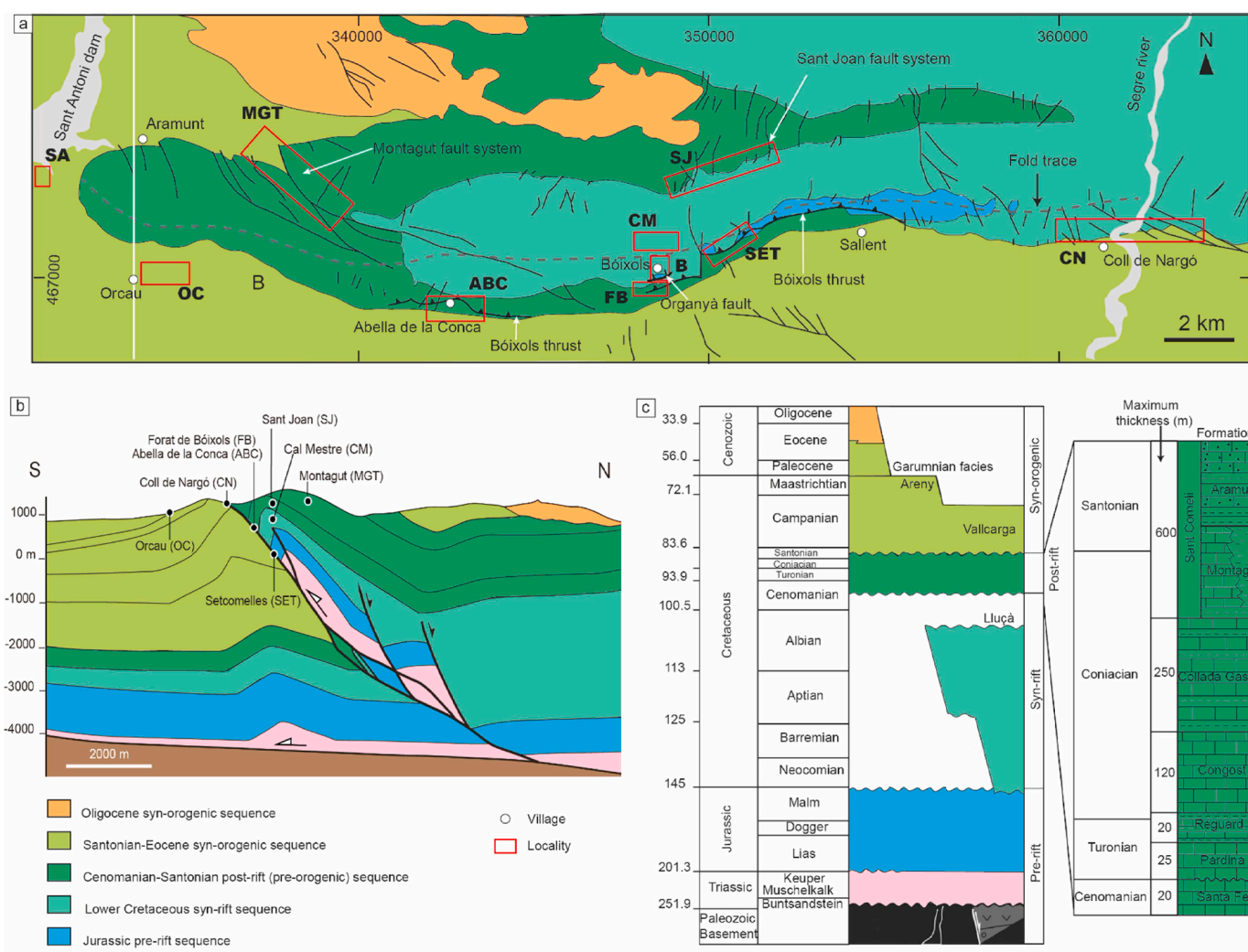
Fig. 2. (a) Simplified geological map (Mencos, 2010; Tavani et al., 2011) and (b) cross-section (Vergés, 1993) of the Bóixols-Sant Corneli anticline showing the studied localities. (c) Chronostratigraphic diagram displaying the main stratigraphic sequences found around the Bóixols-Sant Corneli anticline and their associated tectonic event (Mencos et al., 2015). Location of map and cross-section in Fig. 1a.
