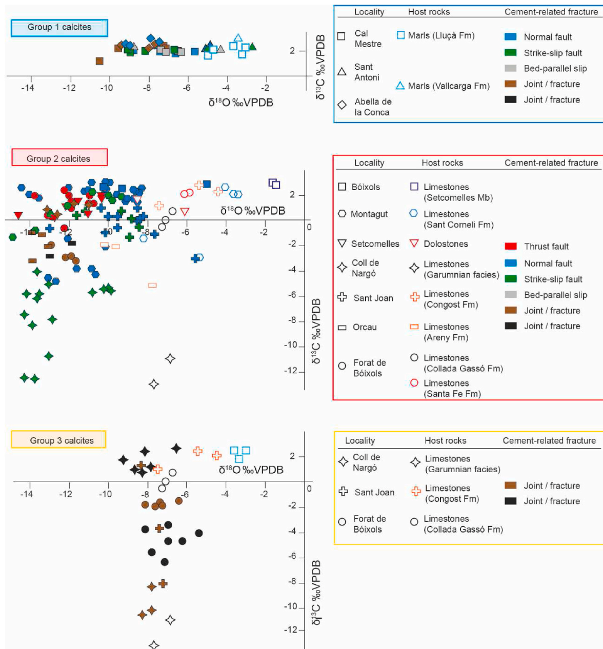
Fig. 7. Stable isotopic composition ( \delta^{18}\text{O} vs \delta^{13}\text{C} ) of the three groups of calcite cements and related host rocks. Solid symbols refer to calcite cements from fractures and open symbols refer to their associated host rocks (the different symbols represent localities where samples were taken).
