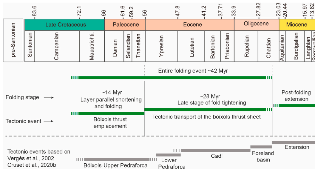
Fig. 11. Age and duration of fold evolution in the Bóixols-Sant Corneli anticline and comparison with the regional deformation of the Bóixols thrust sheet during the evolution of the Southern Pyrenees.
