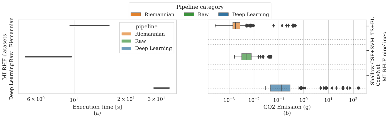
Figure 8: (a) Average execution times in seconds per dataset for the MI right-hand vs feet paradigm, segmented by pipeline category (DL, Riemannian, Raw). (b) Carbon emissions in gCO2 equivalent for the high-ranking pipelines (Raw CSP+SVM, Riemannian TS+EL, DL ShallowConvNet) in the MI right-hand vs feet task.
