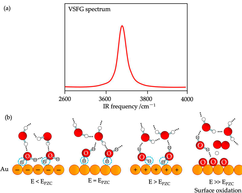
Figure 17. (a) SFG spectrum of non-hydrogen bonded water and (b) its potential-dependent water structure representation. Dotted lines indicate hydrogen bonds. This figure is adapted from reference [254], Copyright © 2017 Wiley.
