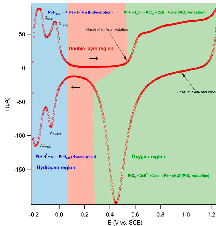
Figure 16. Cyclic voltammogram (CV) of a polycrystalline Pt(poly) electrode in 0.5 M H 2 SO 4 , scan rate: 50 mV·s -1 . While there are three distinctive regions in the Pt(poly) electrode, including the hydrogen region (Pt-H with a strong and a weak adsorption/desorption peak), oxygen region (Pt-OH ad/des and Pt-O ad/des ), and a sandwiched double layer region (ad and d/des are adsorption and desorption, respectively), it appears without hydrogen adsorption/desorption in the Au electrode (only double layer region and oxide region with the formation/reduction of Au oxide species). This figure is obtained from our own CV measurements.
